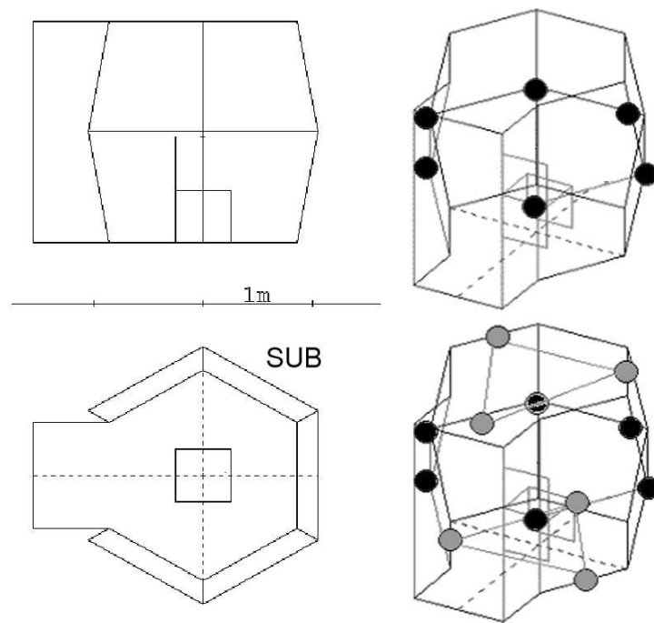
Figure 2: Listening room (adapted from [17]). Loudspeaker locations for the 2-D and 3-D arrays are represented by black dots. A chair is included for reference.
